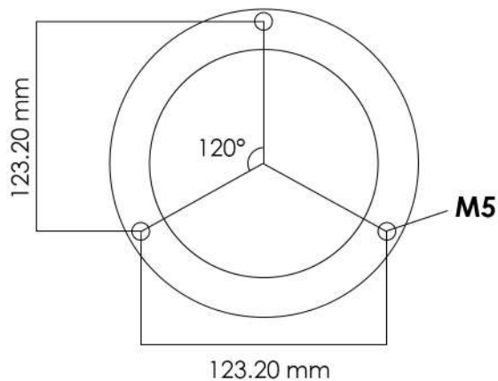
MOUNTING DIAGRAM
