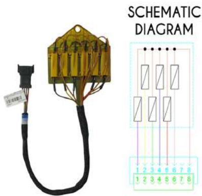
HME-2601090513-01 6 Way Resistor Pack Assembly (12V)
