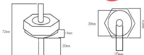
HW2246 Pass Through Stud Kit 3/8"-16 Red
