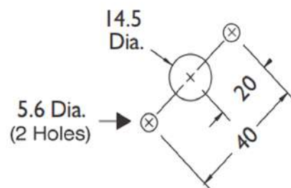
MOUNTING HOLE LAYOUT *M4 Screws
