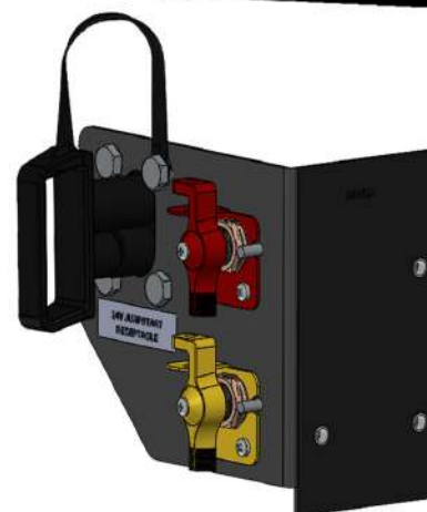
HME-3302090414-01 Left Side Jumpstart Isolator Assy
