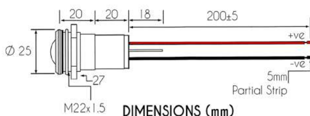
LA1361 LED PANEL INDICATOR WITH LEADS YELLOW RATING: 8-32vdc SIZE: M22
