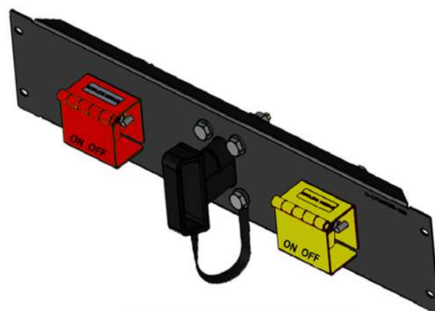
HME-5601090713-01 Mack Jumpstart Isolation Assy
